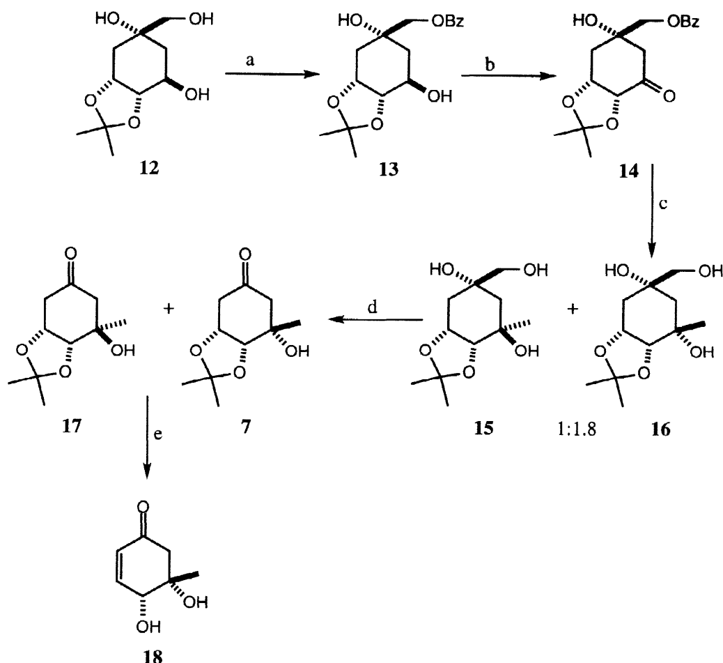
Scheme 2: a) \text{BzCl} , pyridine, 82%. b) periodinane, pyridine, \text{CH}_2\text{Cl}_2 , rt, 88%. c) \text{MeCeCl}_2 , THF, -78^\circ\text{C} . d) \text{NaIO}_4 , \text{H}_2\text{O} , 5 < \text{pH} < 6 . e) \text{NaOH} 0.5 N cat., THF, 0^\circ\text{C} , 60% (3 steps).
