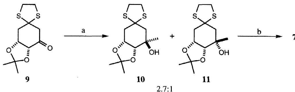
Scheme 1: a) \text{MeCeCl}_2 , THF, -78^\circ\text{C} , 87%. b) \text{HgO}/\text{HgCl}_2 , \text{MeCN}/\text{H}_2\text{O} (8/2), rt, 30%.
