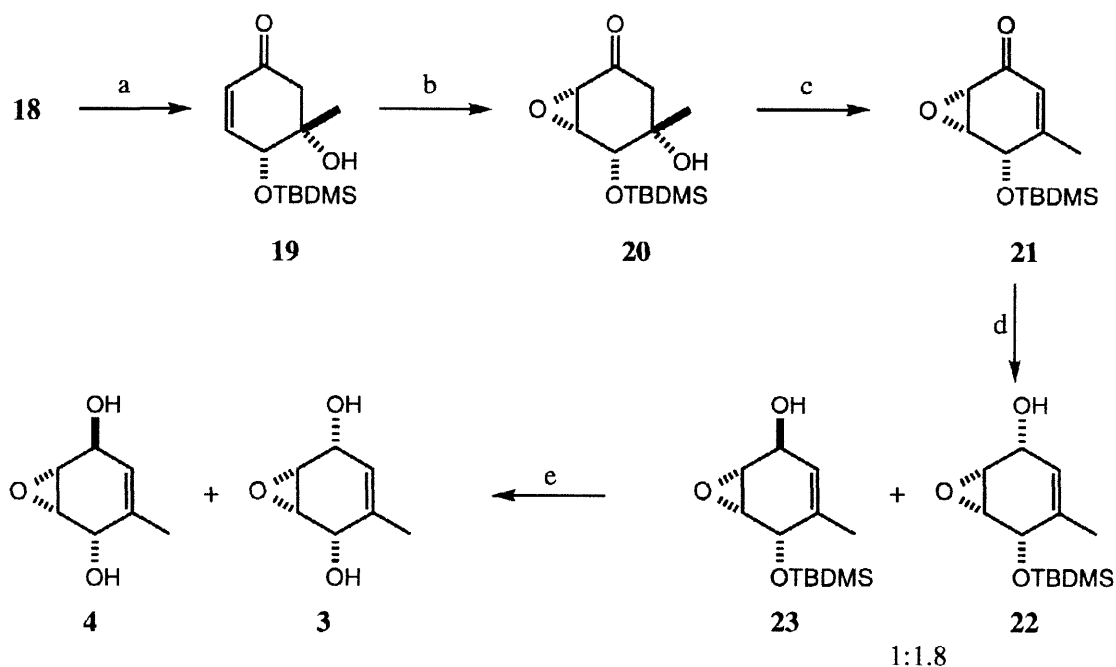
Scheme 3: a) TBDMSCl, DMF, imidazole, rt, 79%. b) H 2 O 2 , Triton B, THF, 0 °C, 92%. c) (CF 3 SO 2 ) 2 O, ( i -Pr) 2 NEt, DMAP, CH 2 Cl 2 , 0 °C, 57%. d) DIBAL-H, THF, -78 °C, 99%. e) Bu 4 NF, THF, H 2 O (trace), rt, 92%.
